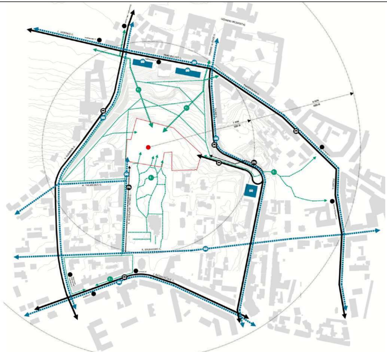
Pav. 10 Eismo organizavimo schema Traffic organisation scheme
