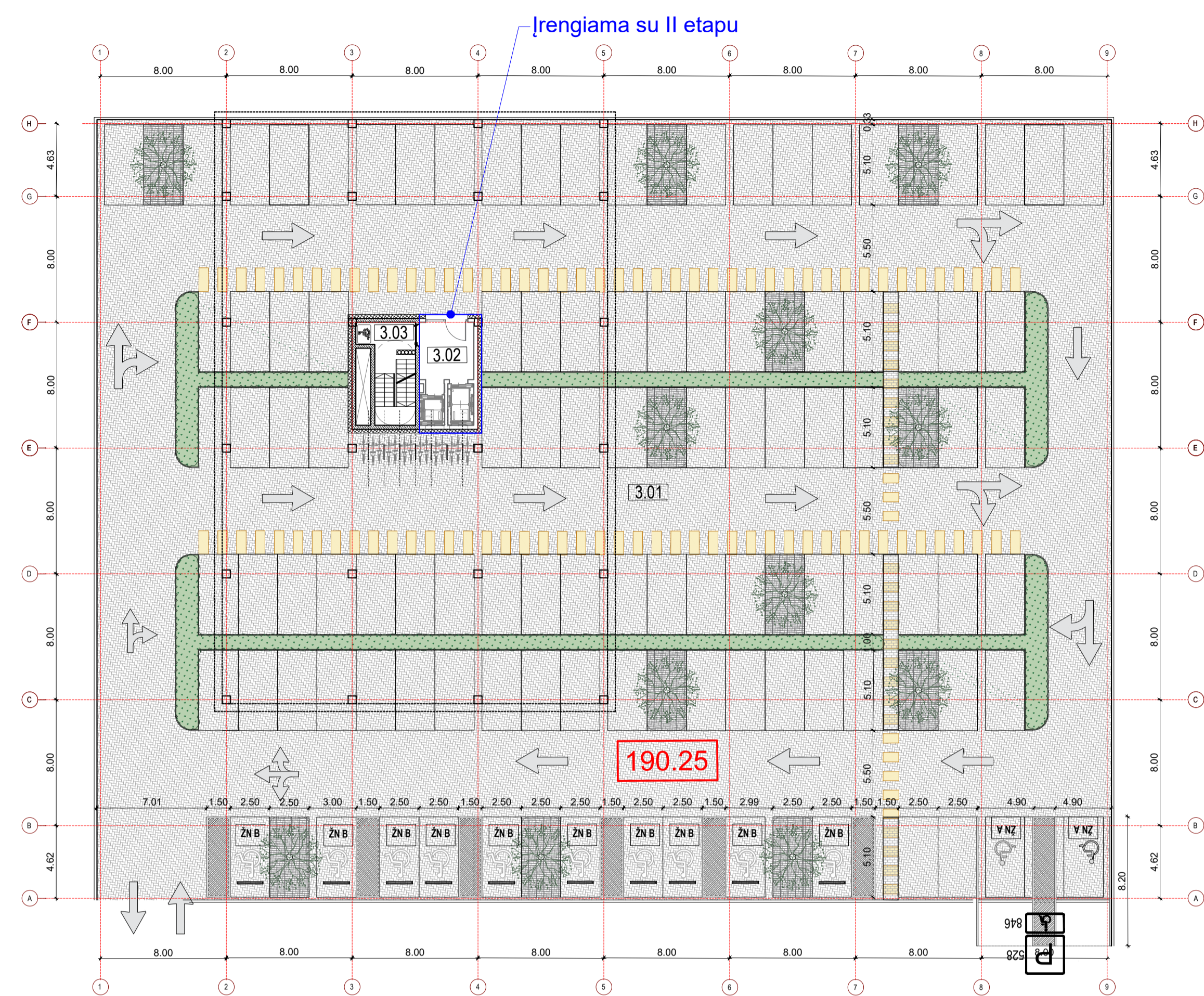
Antrojo parkingo lygio planas
