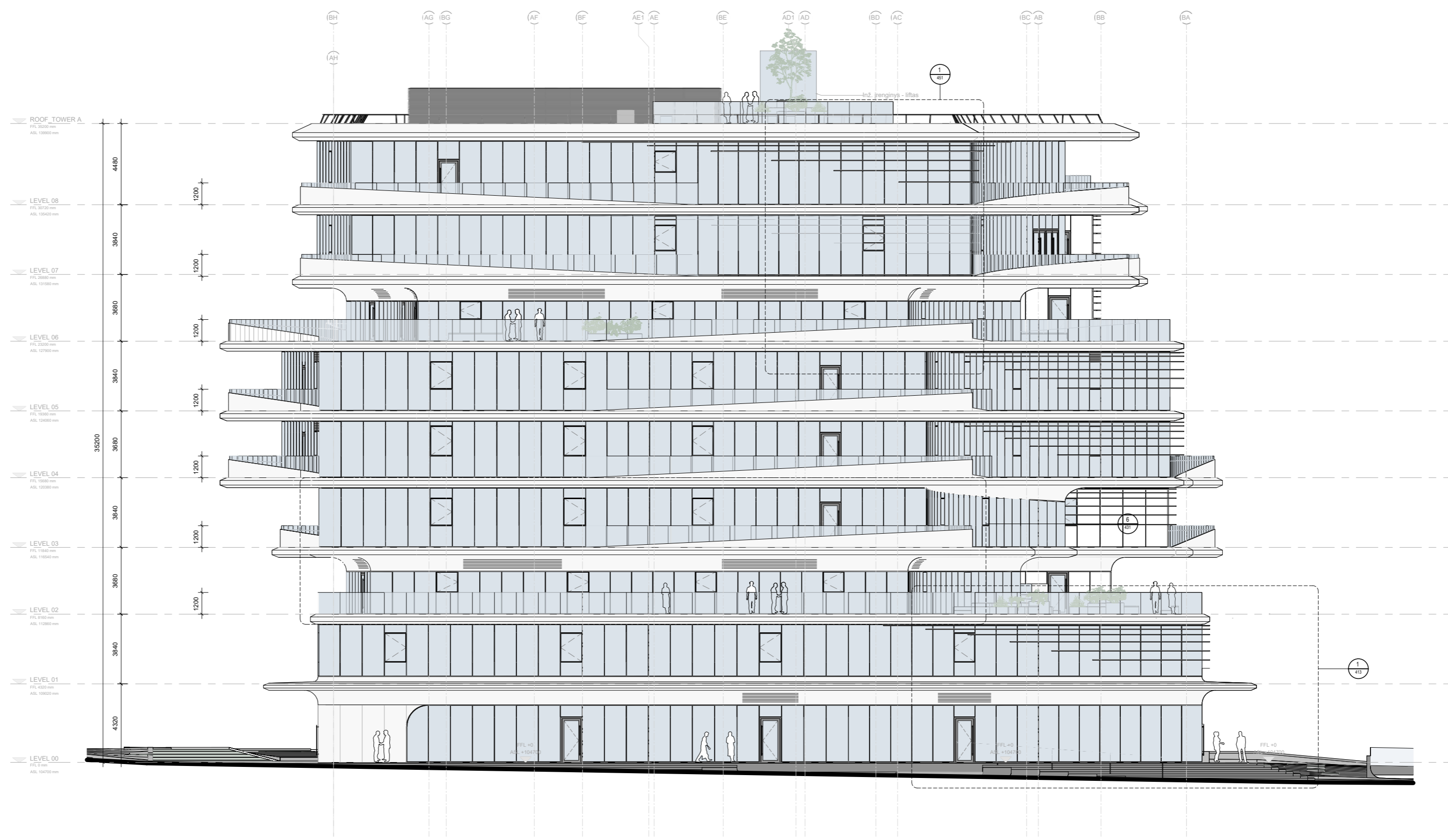
1 Elevation-West
