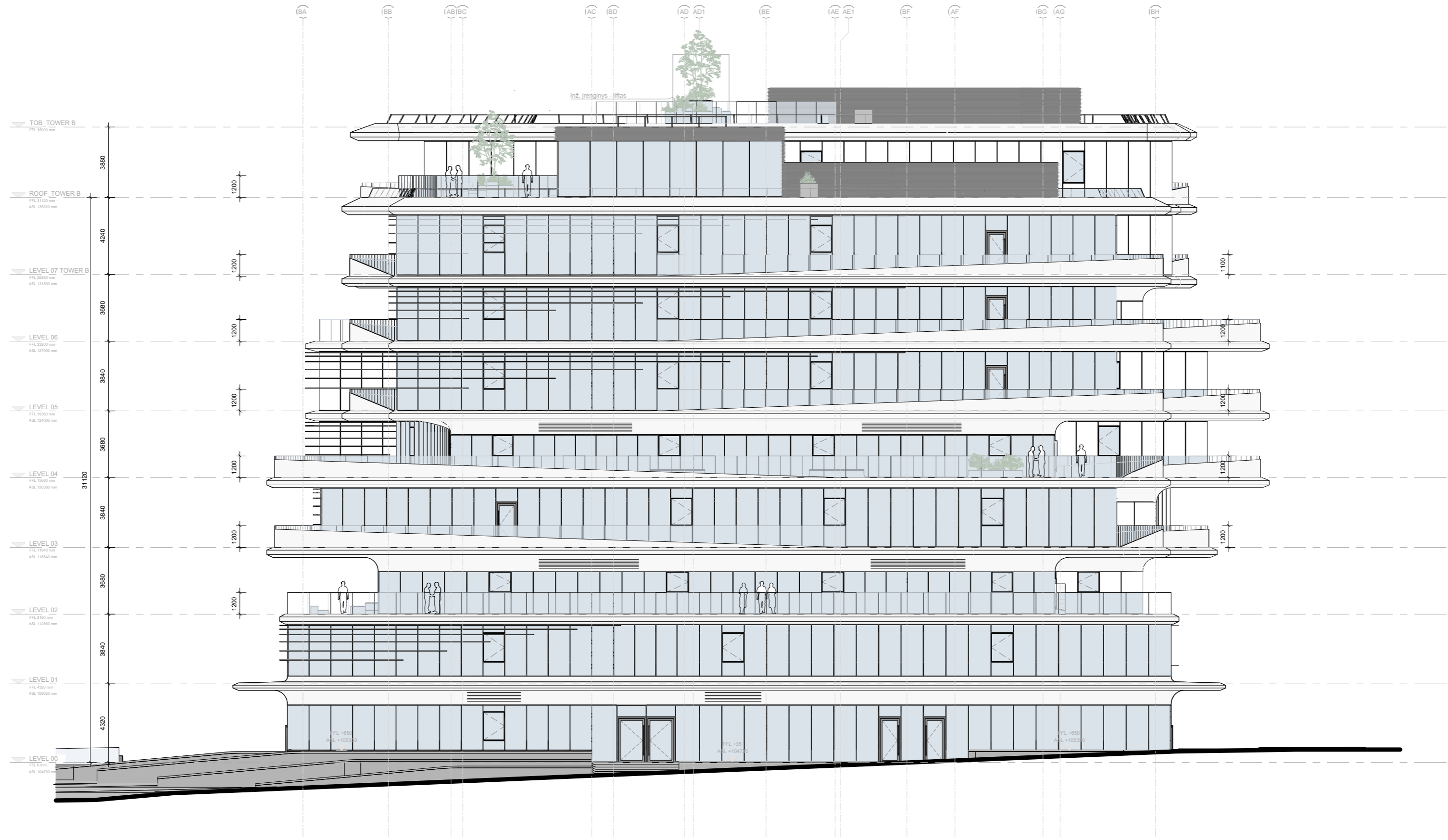
1 Elevation-East 1:100
