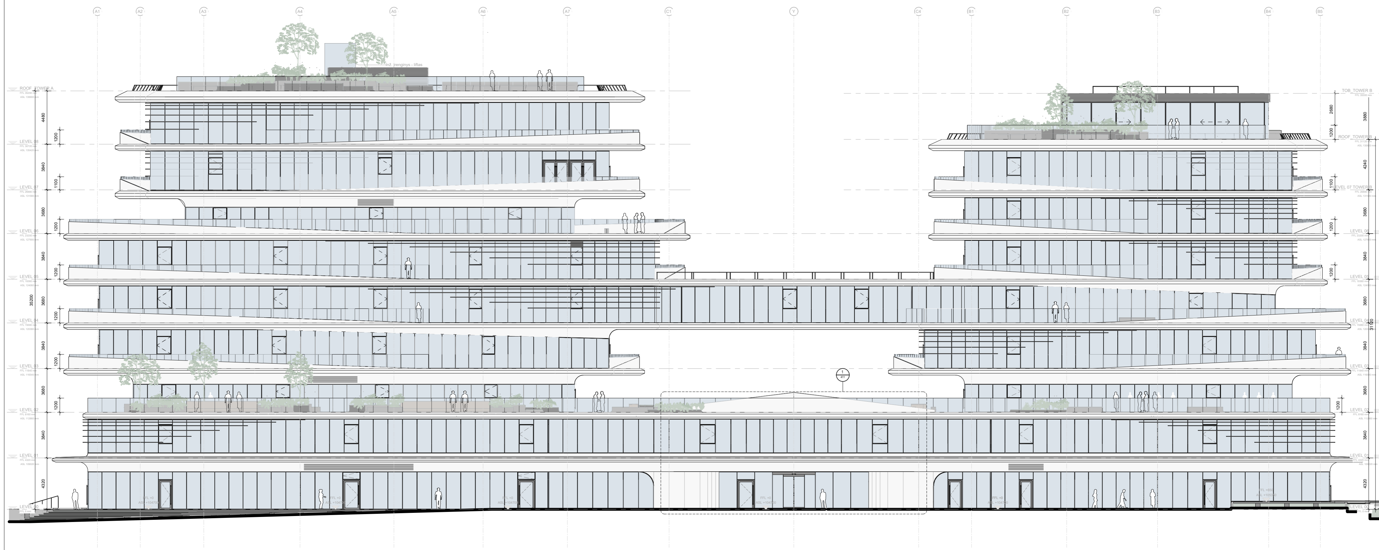
1 Elevation-South 1:100
